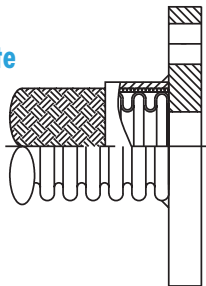
Raised Face Weldneck
