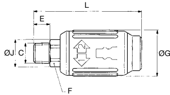
9405U Male Straight Body NPT – 1/4 I.D.
